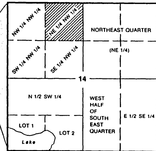
SECTION 14
